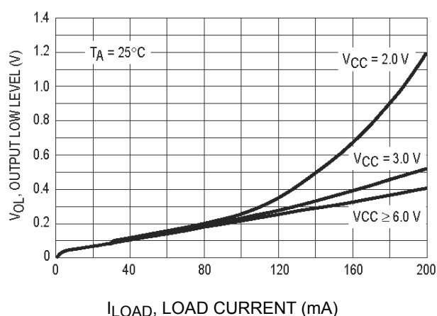
Figure 19. V_{OL} @ V_{O1} , V_{O2} versus Load Current
