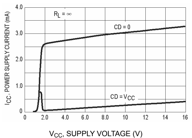
Figure 15. Power Supply Current
