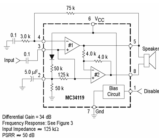
Figure 21. Audio Amplifier with High Input Impedance
