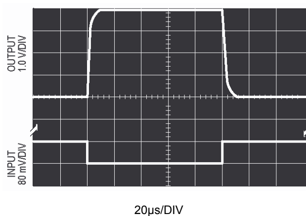
Figure 17. Large Signal Response
