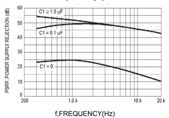
Figure 5. Power Supply Rejection versus Frequency (C2 = 5.0 \mu F)
