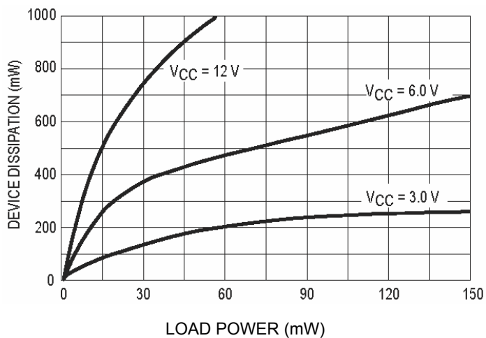
Figure 8. Device Dissipation, 8.0 \Omega Load
