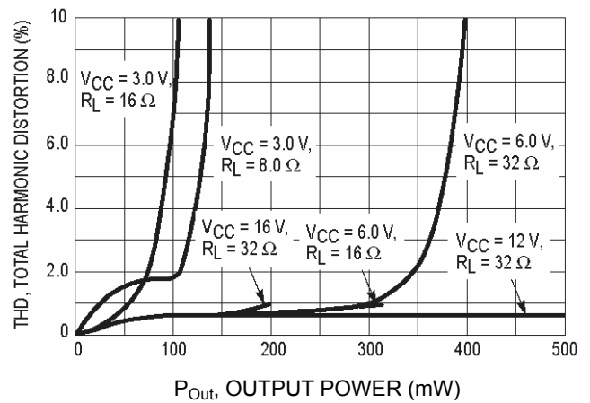
Figure 13. Distortion versus Power
